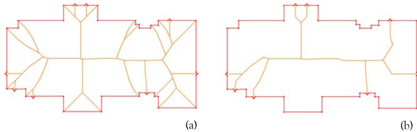
Fig.3-4: (a) Exact medial axis of a typical room contour. Spikes in the contour are portal positions. (b) Trimmed to remove branches that do not lead to portals.
