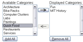
Fig.4.4: Alternative “K of N” widget for category selection – one list box for the K selected choices, the other listing all N choices.
