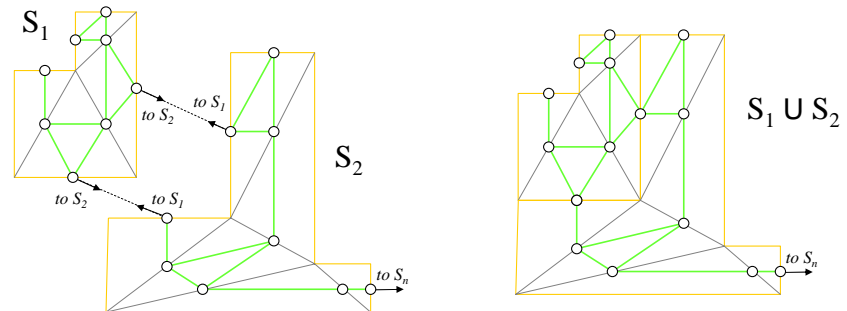
Fig.3-7: Combination of internal graphs for spaces S_1 and S_2 . Green lines are graph edges, solid circles are graph nodes, and gray lines are space triangulations. Nodes incident on the space contour represent portals. The two graphs are connected at corresponding portal nodes.
