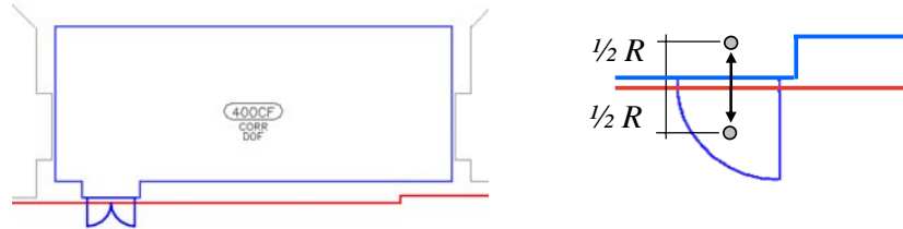
Fig.2-13: Explicit inter-building portal. A point is placed on either side of the door frame. One point is contained by the portal's source space, the other lies outside the floor contour (red line).
