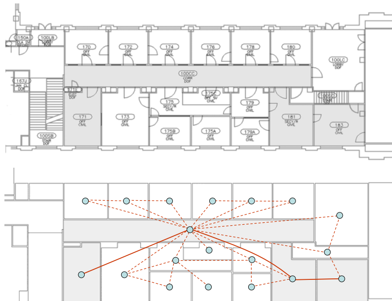
Fig.3-2: Sample space-portal graph. Edges are placed between adjacent spaces, and weights are calculated as the distance between space centroids.
