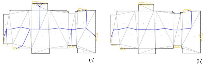
Fig.3-5: (a) Approximate medial axis of a room contour, connecting midpoints of shared triangles edges; (b) Example of one intra-space path.
