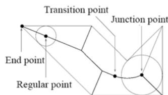
Fig.1-9: Taxonomy of medial axis points [Joan-Arinyo 1996].
