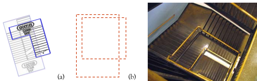
Fig.2-11: Vertical portal. (a) Plan view of stairs on adjacent floors; (b) axis-aligned bounding box for each stair space. Matches are made by testing for overlapping bounding boxes.
