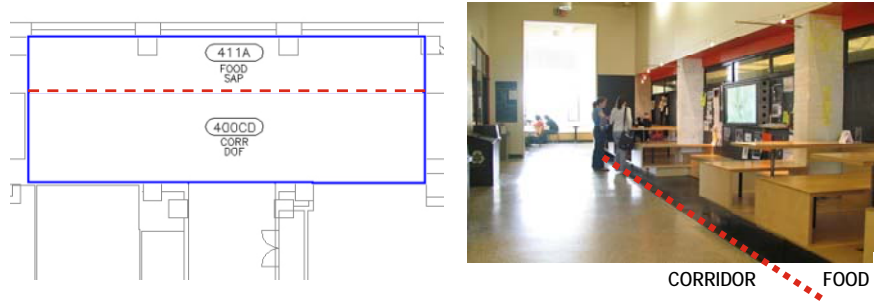
Fig.2-10: A sample implicit portal. The dotted line denotes an incident edge between the space contours. Although no physical barrier exists, the portal places an implicit divide between the corridor and café tables.
