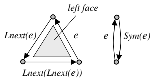
Fig.1-11: Basic edge functions.
